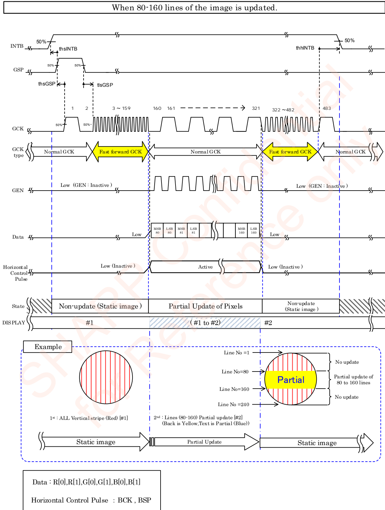
Figure 6-5-4 Partial update Sequence (Reference Specification)
