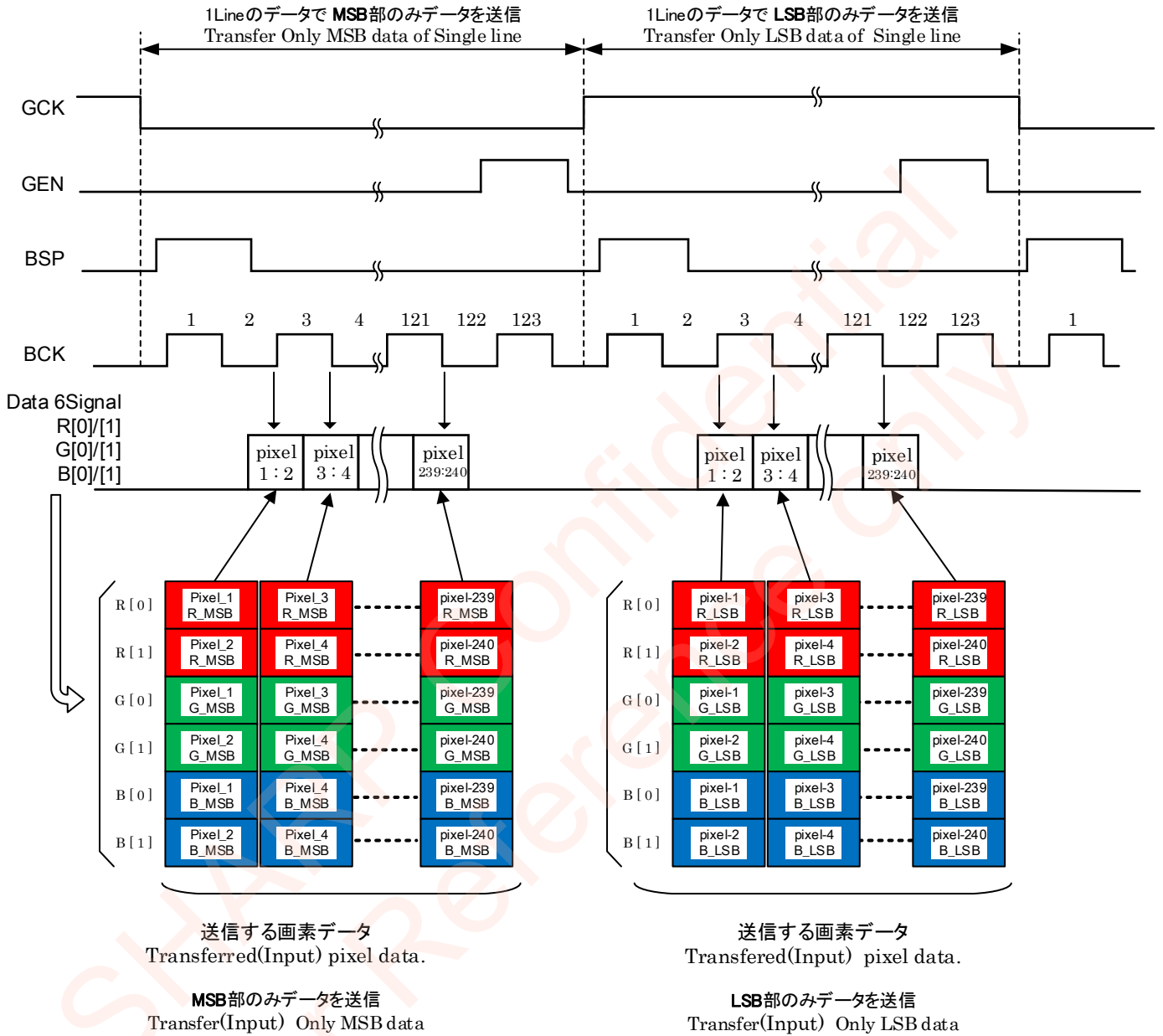
Figure 6-5-2 Horizontal Diagram
